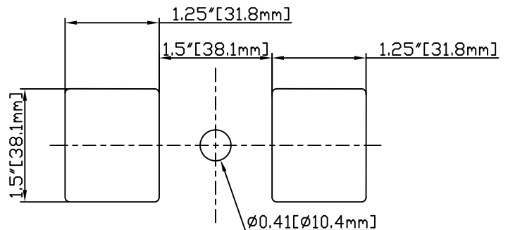
PARTIAL VIEW
